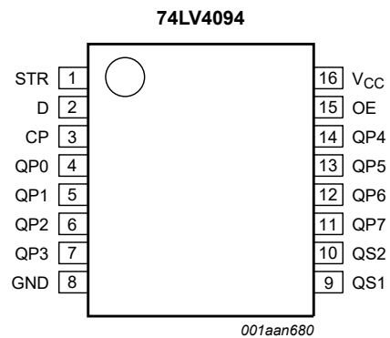
Fig. 6. Pin configuration SOT338-1 (SSOP16) and SOT403-1 (TSSOP16)
